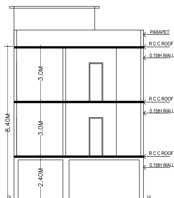
SECTION @X-X
